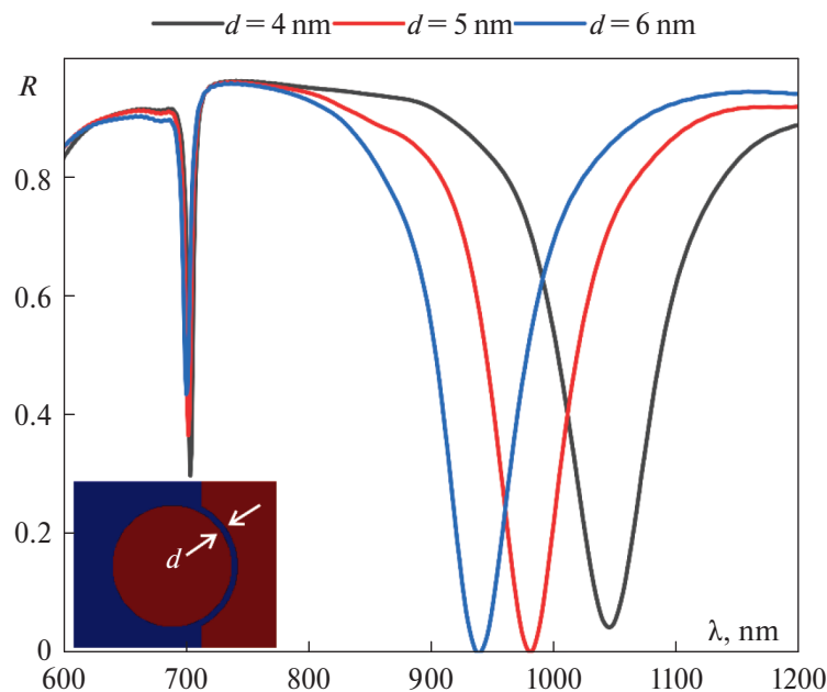
Fig. 4. Calculated reflectivity spectra of the NA array for three widths of the gap between the NA and substrate material: d = 4 , 5 , and 6 nm. Other parameters are as follows: n_0 = 1 , h = 25 nm, r = 50 nm, T = 700 nm.
