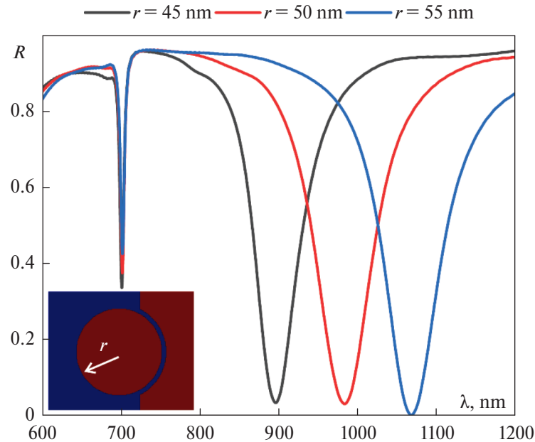
Fig. 2. Calculated reflectivity spectra of the NA array for three values of the NA radius: r = 45, 50 , and 55 nm. Other parameters are as follows: n_0 = 1 , d = 5 nm, h = 25 nm, T = 700 nm.
