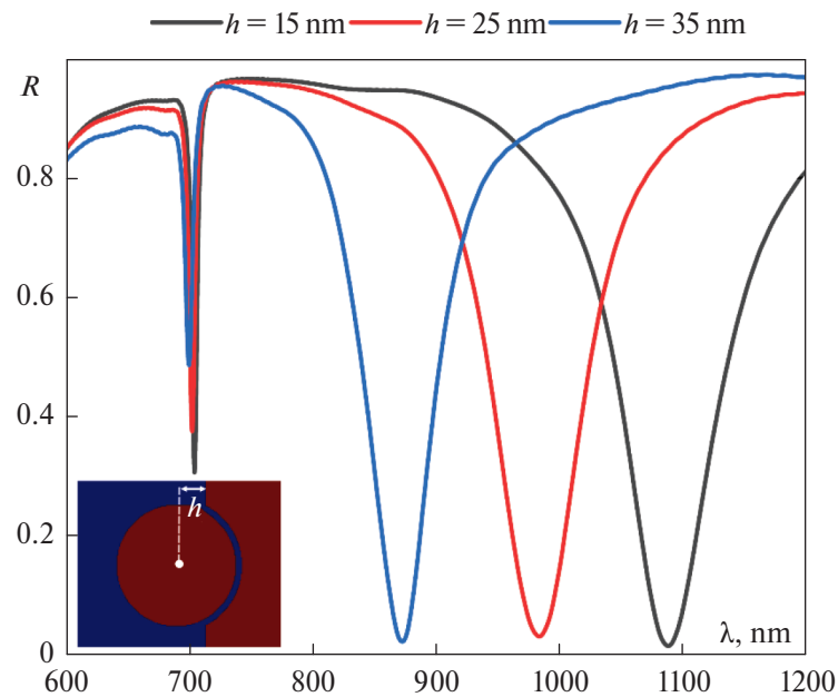
Fig. 3. Calculated reflectivity spectra of the NA array for three values of the NA burial depth: h = 15 , 25 , and 35 nm. Other parameters are as follows: n_0 = 1 , d = 5 nm, r = 50 nm, T = 700 nm.
