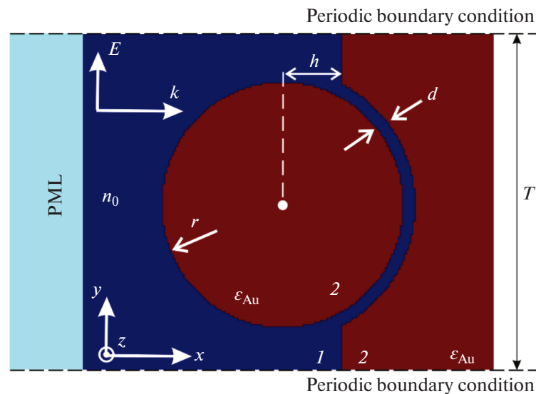
Fig. 1. Schematic drawing of the unit cell of the NA array and its parameters (1—dielectric medium with refractive index n_0 , 2—gold with dielectric permittivity \epsilon_{\text{Au}} ).
