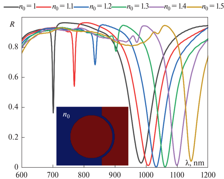
Fig. 8. Calculated reflectivity spectra of the NA array for various values of the refractive index of the ambient dielectric medium: n_0 = 1, 1.1, 1.2, 1.3, 1.4 , and 1.5 . Other parameters are as follows: h = 25 nm, r = 50 nm, d = 5 nm, T = 700 nm.
