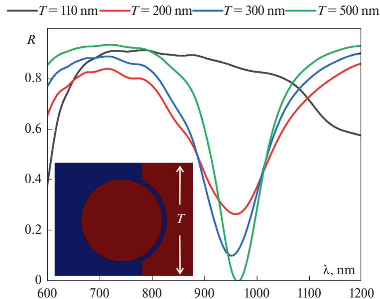
Fig. 7. Calculated reflectivity spectra of the NA array for various (small) periods of the array T = 110, 200, 300 , and 500 nm. Other parameters are as follows: n_0 = 1 , h = 25 nm, r = 50 nm, d = 5 nm.
