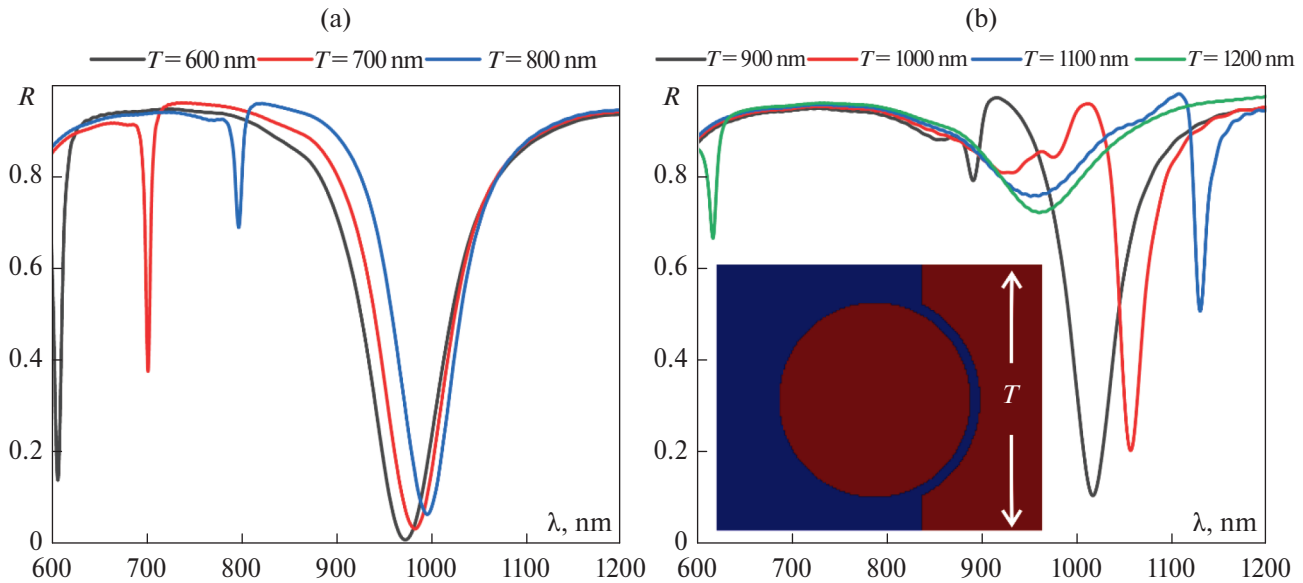
Fig. 5. Calculated reflectivity spectra of the NA array for various periods of the array. Illustrated in the two panels are the cases when the array resonance and the nanoantenna resonances do not (Fig 5a, T = 600, 700 and 800 nm) and do (Fig 5b, T = 900, 1000, 1100 , and 1200 nm) overlap. Other parameters are as follows: n_0 = 1 , h = 25 nm, r = 50 nm, d = 5 nm.
