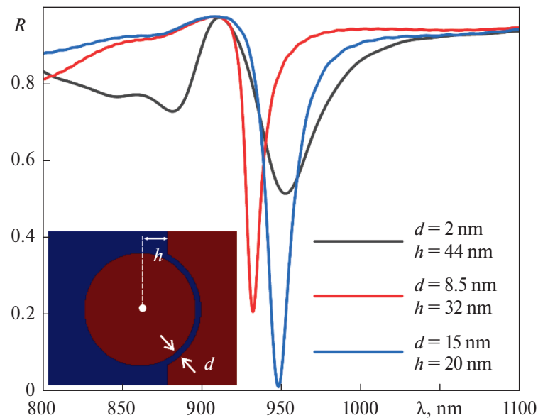
Fig. 6. Calculated reflectivity spectra of the NA array for three combinations of the gap width between the NA and substrate material and NA burial depth: d = 2 nm, h = 44 nm; d = 8.5 nm, h = 32 nm; d = 15 nm, h = 20 nm. The combinations are chosen so as to keep the AR and NAR overlapped. Other parameters are as follows: n_0 = 1 , r = 50 nm, T = 900 nm.
