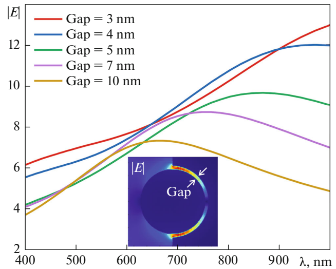
Fig. 4. Spectral dependences of the maximum electric field amplitude for the sphere \sim 50\% buried in the substrate with various gap width ranging from 3 to 10 nm, R = 50 nm.
