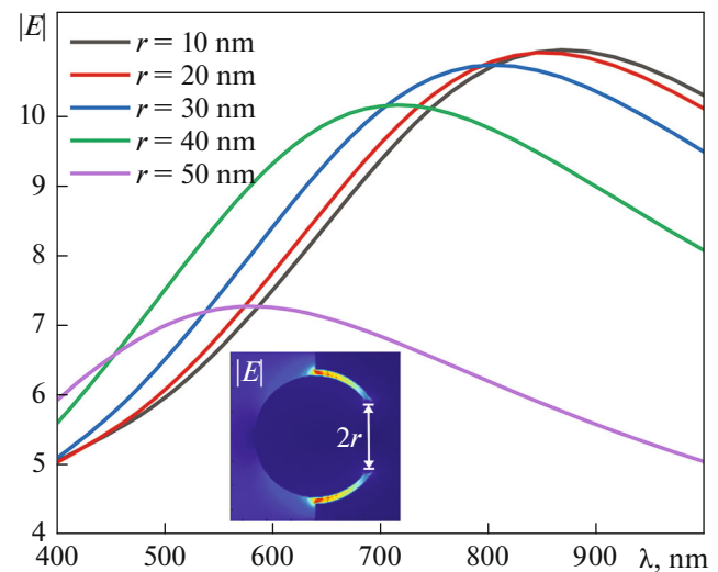
Fig. 5. Spectral dependences of the maximum electric field amplitude for the sphere with R = 50 nm, \sim 50\% buried in the substrate with a gap of 5 nm and attached to the substrate with a cylindrical nickel stem of various radii.
