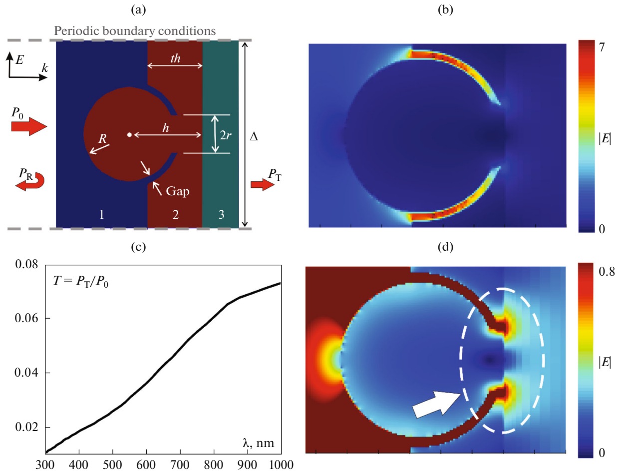
Fig. 6. Numerical simulation results for a nickel film on a glass substrate with defects in the form of nickel spheres partly buried in the film: (a) simulated geometry in side view ((1) vacuum, (2) nickel, (3) glass substrate, R = 50 nm, gap = 5 nm, r = 20 nm, h = 54 nm, th = 60 nm, \Delta = 130 nm); (b) distribution of the electric field amplitude in the plane of the E vector at \lambda = 1000 nm; (c) calculated transmission spectrum of the nickel film with defects; (d) distribution of the electric field amplitude at \lambda = 1000 nm with a changed color scale to make the leaking of the electromagnetic field from the gaps into the glass clearly visible.
