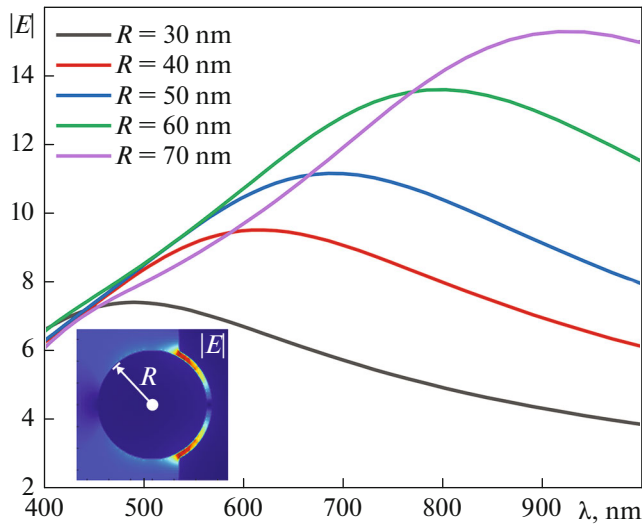
Fig. 3. Spectral dependences of the maximum electric field amplitude for various radii of the sphere \sim 25\% buried in the substrate with a gap of 5 nm.
