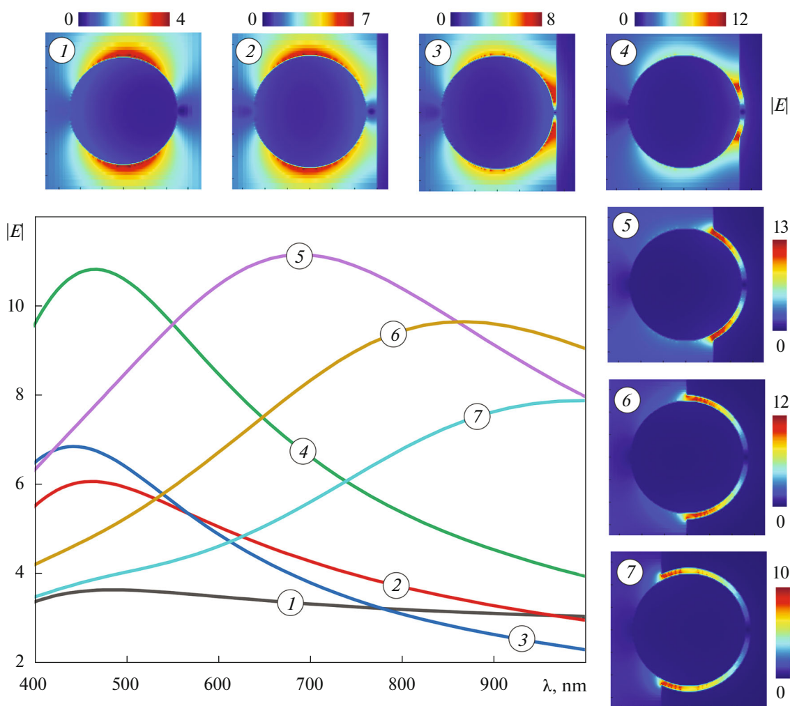
Fig. 2. Spectral dependences of the maximum electric field amplitude (in a point near the sphere where it is the strongest) for various locations of the R = 50 nm nickel sphere with respect to the nickel substrate: (1) isolated sphere in a vacuum without the substrate, (2) sphere with a separation of 10 nm between its surface and the substrate, (3) same as (2), but the separation is 3 nm. Curves 4–7 are for the sphere imbedded in the substrate with a 5 nm gap: h = (4) 50, (5) 25, (6) 0, and (7) –25 nm. Shown in the correspondingly numbered insets are the distributions of the electric field amplitude at the resonant wavelengths (when the near field around the sphere is the strongest).
