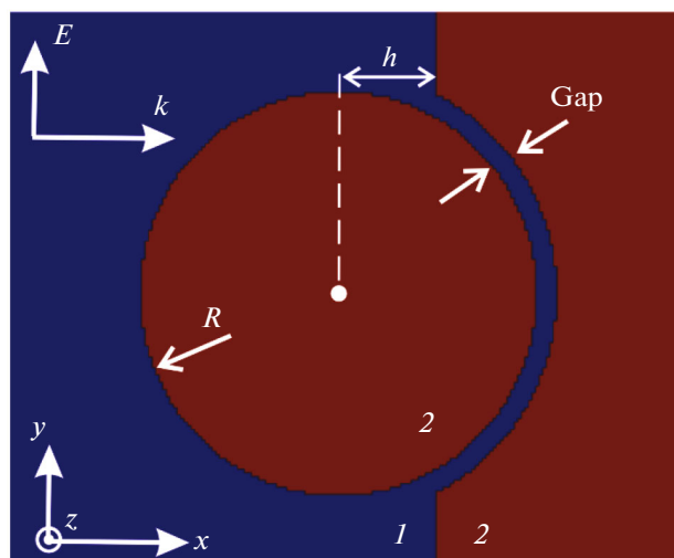
Fig. 1. Schematic drawing of the arrangement under study and its parameters (1—vacuum, 2—nickel).
