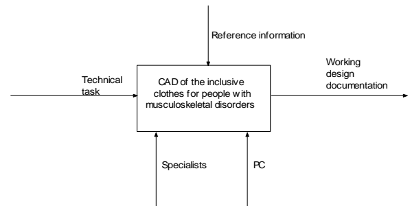
Figure 1 - The inclusive clothing CAD IDEF0-model's FEO diagram (level 1)
